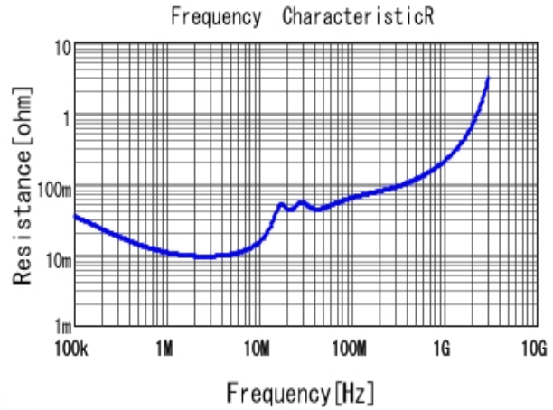
■ GCJ43DR72E474KXJ1 R DC0V, 25degC
