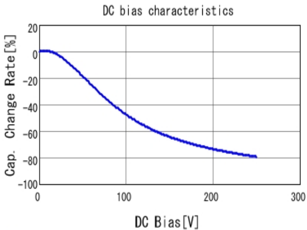
■ GCJ43DR72E474KXJ1 C-DC bias capchange, 25.0degC, AC1V
