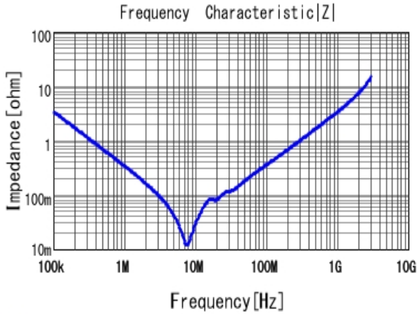
■ GCJ43DR72E474KXJ1 |Z| DC0V, 25degC
