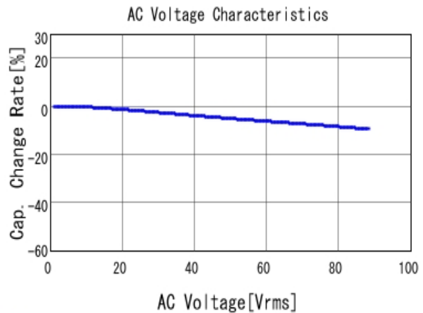
■ GCJ43DR72E474KXJ1 C-AC Voltage capchange, DC0V, 25.0d
