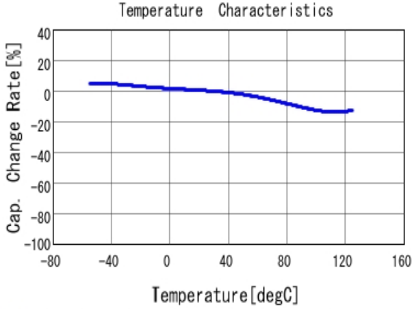
■ GCJ43DR72E474KXJ1 C-Temp. capchange, DCOV, AC1Vrms
