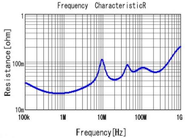
■ RDER72J474MUE1H03A R DCOV, 25degC
