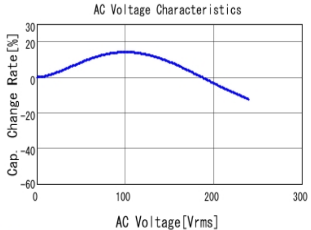
■ RDER72J474MUE1H03A C-AC Voltage capchange, DCOV, 25.0
