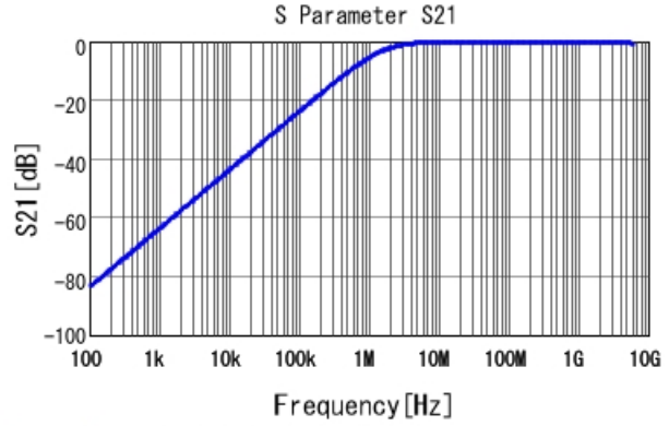
GCM188R71E102KA37 S21 DC0V, 25degC
