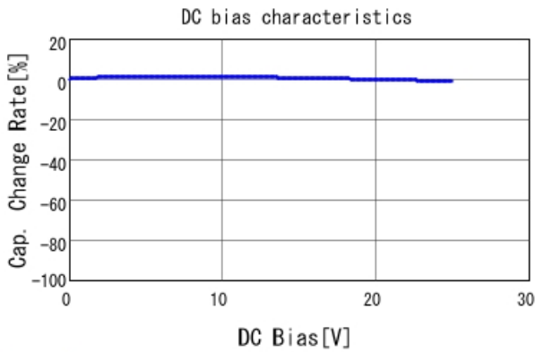
GCM188R71E102KA37 C-DC bias capchange, 25.0degC, A
