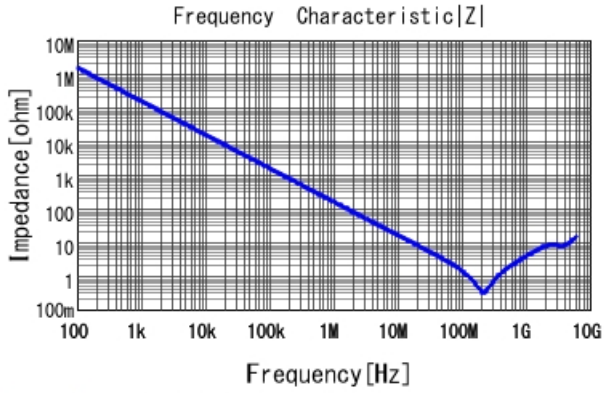
GCM188R71E102KA37 |Z| DCOV, 25degC
