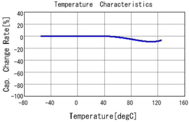
GCM188R71E102KA37 C-Temp. capchange, DC0.0V, AC1.C
