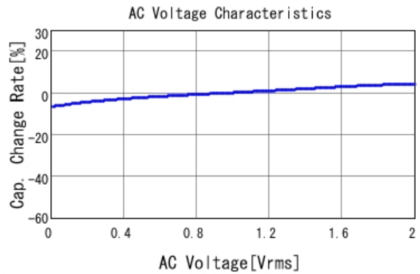
GCM188R71E102KA37 C-AC Voltage capchange, DCOV, 25
