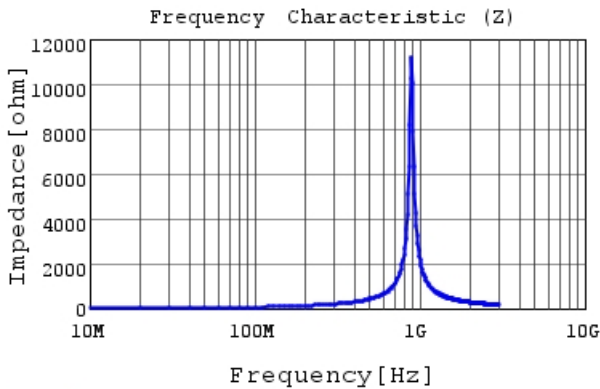
LQG15HZR10G02 |Z|
