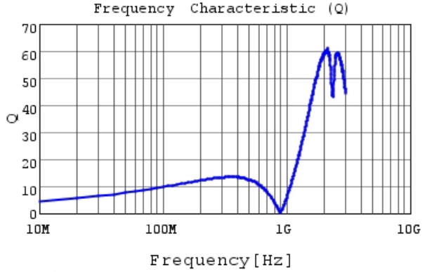
LQG15HZR10G02 Q
