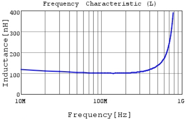
LQG15HZR10G02 L
