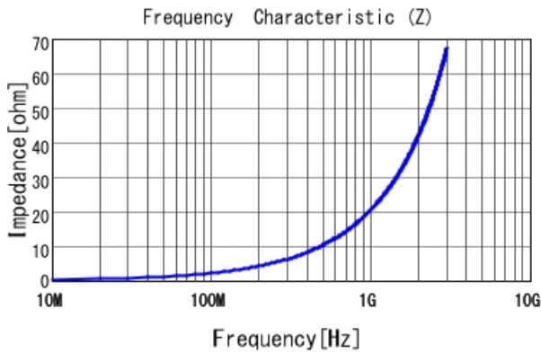
LQP03TN3N3BZ2 |Z|
