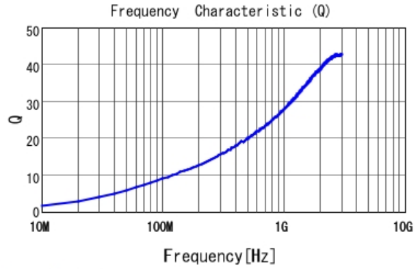
LQP03TN3N3BZ2 Q
