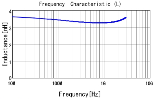
LQP03TN3N3BZ2 L
