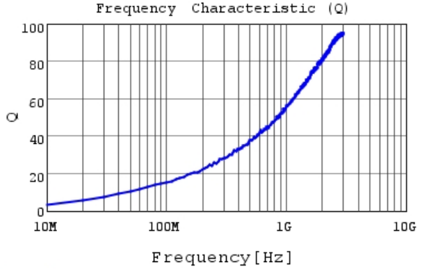
LQG15WZ2N0S02 Q
