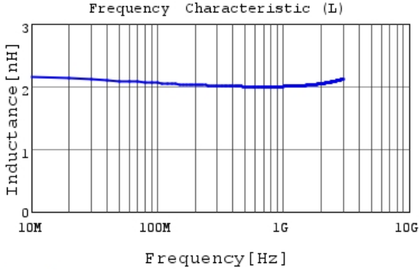
LQG15WZ2N0S02 L
