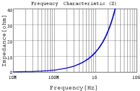
LQG15WZ2N0S02 |Z|
