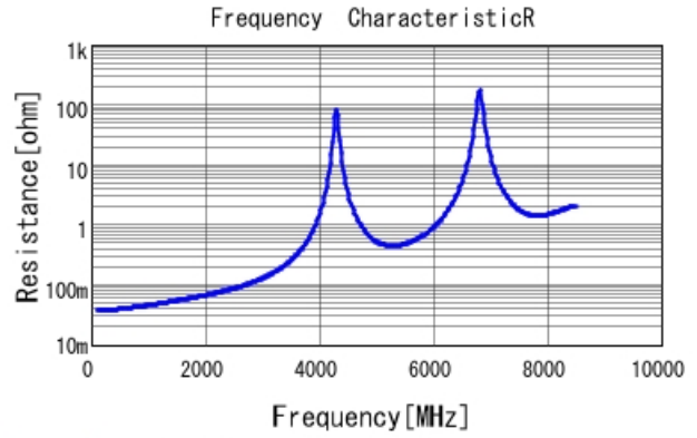
GQM2195C2E150JB12 R DCOV, 25degC
