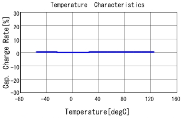
GQM2195C2E150JB12 C-Temp. capchange, DCOV, AC1Vrms
