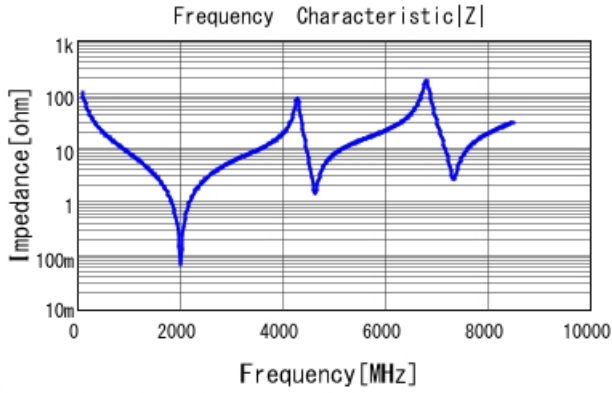
GQM2195C2E150JB12 |Z| DCOV, 25degC
