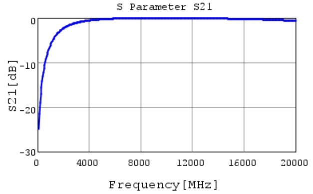
GJM0335C1ER90BB01 S21 DCOV, 25degC
