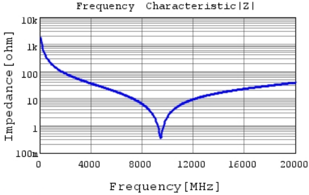
GJM0335C1ER90BB01 |Z| DCOV, 25degC
