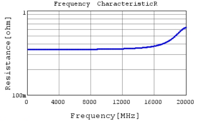
GJM0335C1ER90BB01 R DCOV, 25degC
