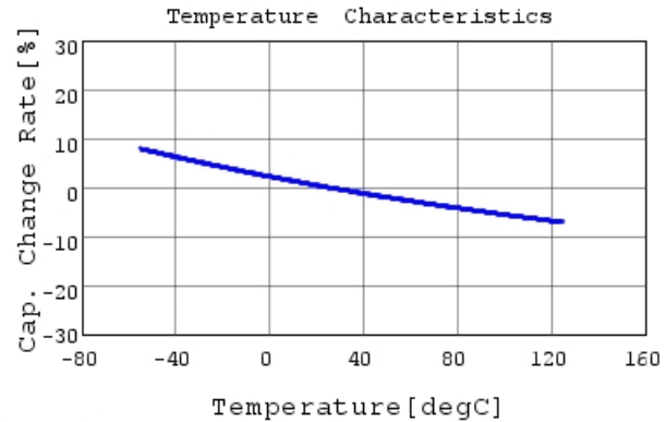
GRM31A7U2J470JW31 C-Temp. capchange, DC0V, 1
