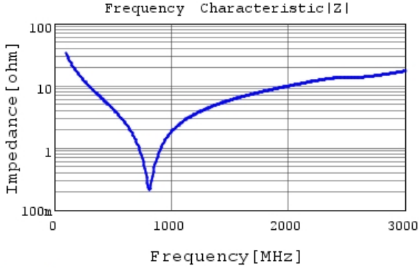
GRM31A7U2J470JW31 |Z| DC0V, 25degC
