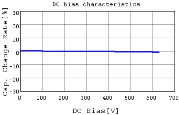
GRM31A7U2J470JW31 C-DC bias capchange, 25.0c
