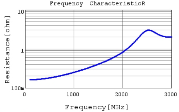
GRM31A7U2J470JW31 R DC0V, 25degC
