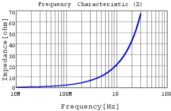
LQP15MN3N3W02 |Z|
