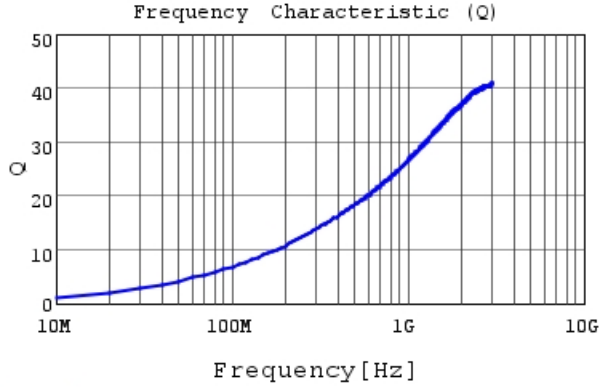
LQP15MN3N3W02 Q
