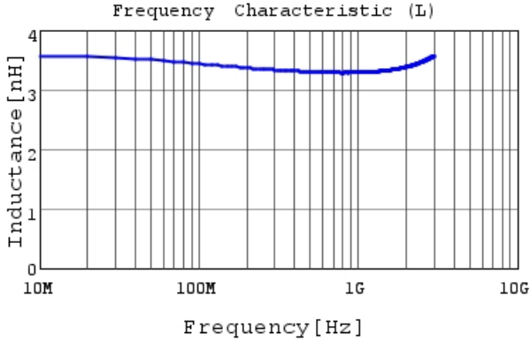
LQP15MN3N3W02 L
