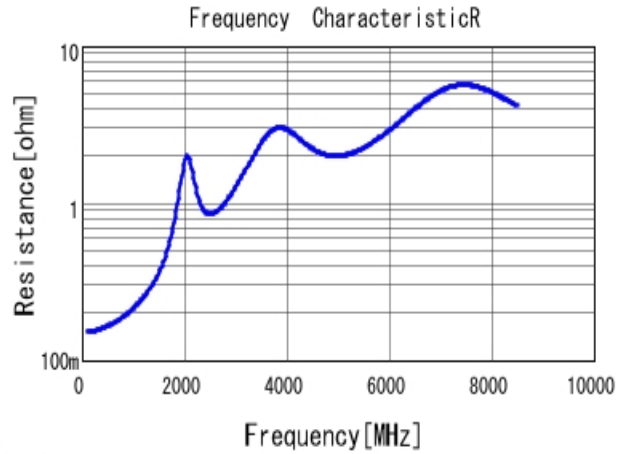
■ GRM1885C1H470JA01 R DCOV, 25degC
