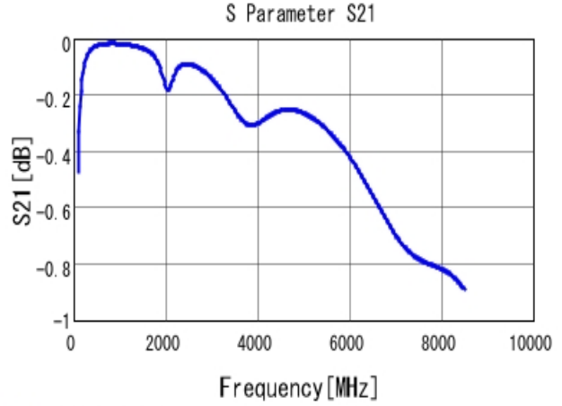
■ GRM1885C1H470JA01 S21 DCOV, 25degC
