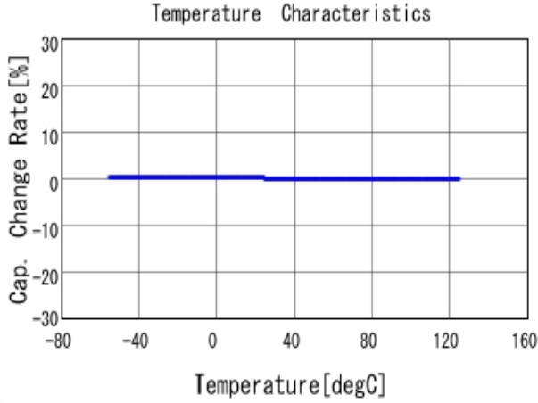
■ GRM1885C1H470JA01 C-Temp. capchange, DCOV, AC1Vrms
