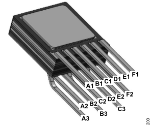
Figure 4. Pin Configuration (3D View)
