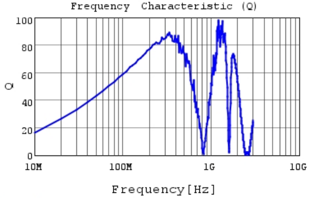
LQW2UASR22F00 Q
