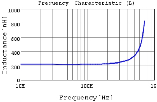
LQW2UASR22F00 L
