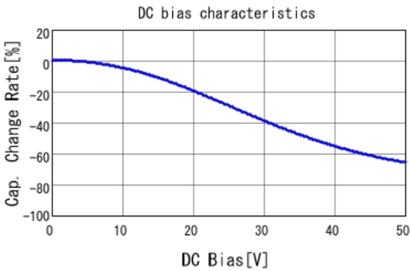
GRM31MR71H684KA88 C-DC bias capchange, 25.0degC, A
