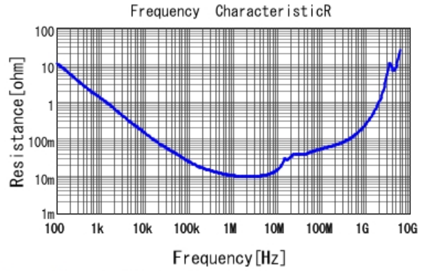
GRM31MR71H684KA88 R DCOV, 25degC
