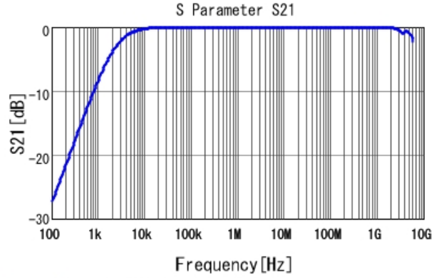
GRM31MR71H684KA88 S21 DCOV, 25degC
