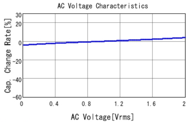
GRM31MR71H684KA88 C-AC Voltage capchange, DCOV, 25
