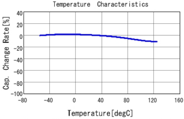
GRM31MR71H684KA88 C-Temp. capchange, DCO. 0V, AC1. C
