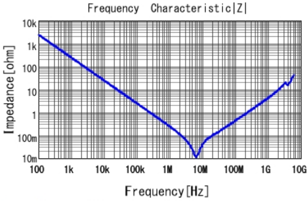
GRM31MR71H684KA88 |Z| DCOV, 25degC
