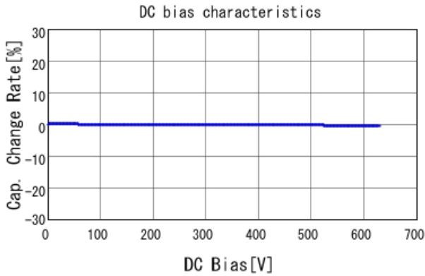
■ GRM21B5C2J182JWAA C-DC bias capchange, 25.0degC, AC1V
