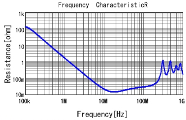
■ GRM21B5C2J182JWAA R DCOV, 25degC
