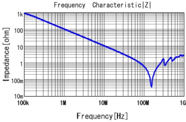
■ GRM21B5C2J182JWAA |Z| DCOV, 25degC
