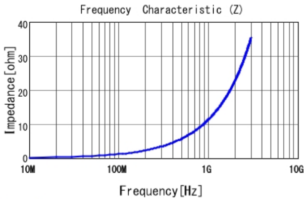
LQP03TN1N8B02 |Z|
