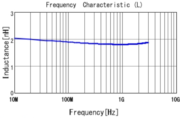
LQP03TN1N8B02 L
