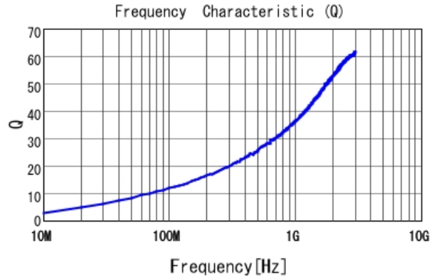
LQP03TN1N8B02 Q
