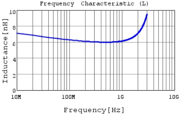
LQG15HZ6N2S02 L
