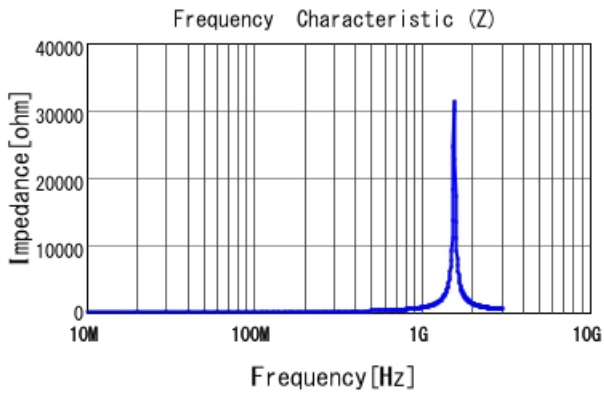
LQG15WZ72NG02 |Z|
