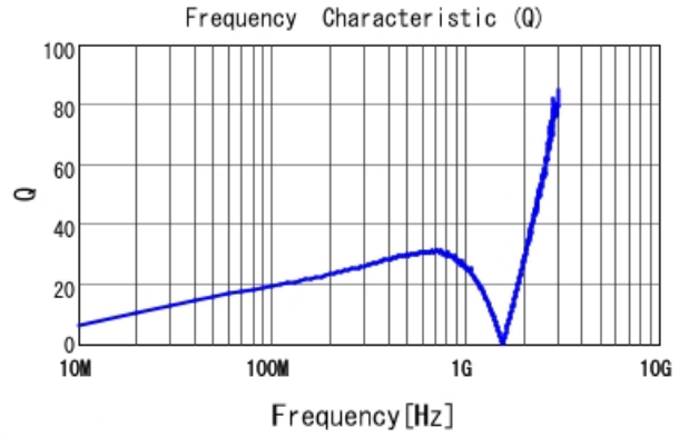
LQG15WZ72NG02 Q
