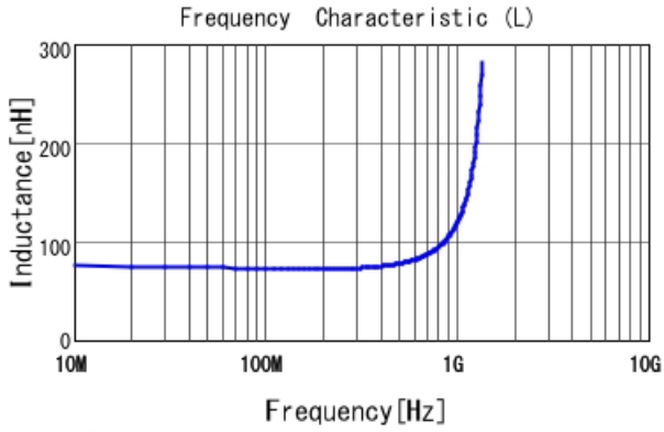
LQG15WZ72NG02 L
