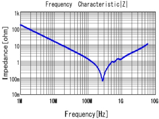
■ GRM1555C1H102JA01 |Z| DCOV, 25degC
