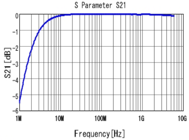
■ GRM1555C1H102JA01 S21 DCOV, 25degC
