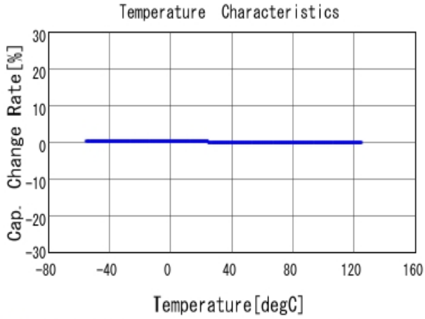
■ GRM1555C1H102JA01 C-Temp. capchange, DCOV, AC1Vrms
