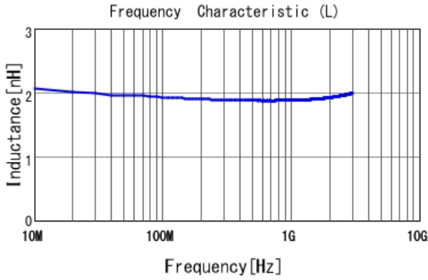
LQG15WH1N9S02 L
