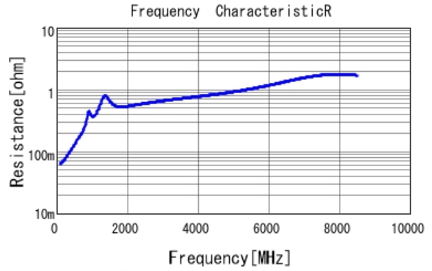
GRM1552C1H391JA01 R DCOV, 20degC
