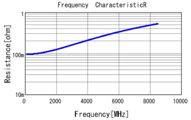
GJM0335C1E4R5WB01 R DCOV, 25degC
