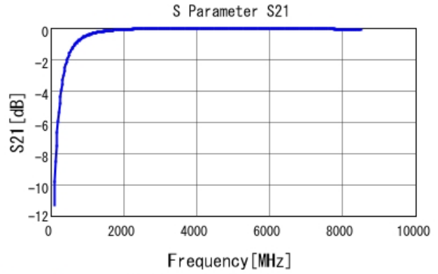
GJM0335C1E4R5WB01 S21 DC0V, 25degC
