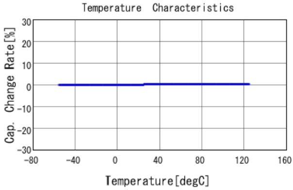
GJM0335C1E4R5WB01 C-Temp. capchange, DC0V, AC1Vrms
