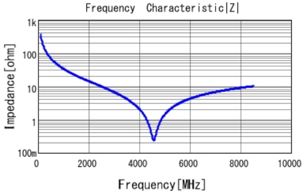
GJM0335C1E4R5WB01 |Z| DCOV, 25degC
