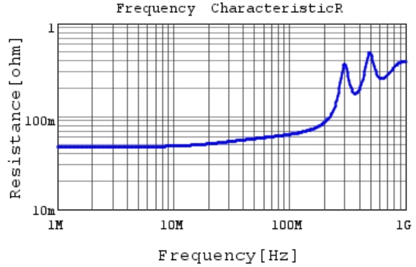
RCE5C1H222J0M1H03A R DCOV, 25degC
