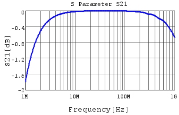
RCE5C1H222J0M1H03A S21 DC0V, 25degC
