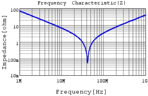
RCE5C1H222J0M1H03A |Z| DCOV, 25degC
