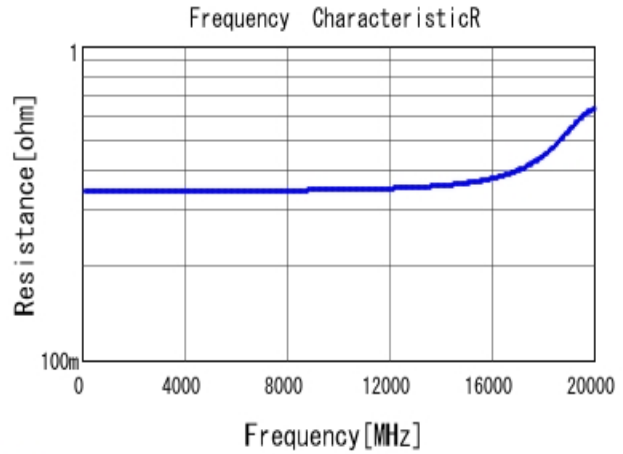
■ GJM0335C1HR90WB01 R DC0V, 25degC
