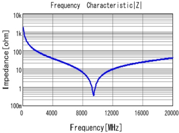
■ GJM0335C1HR90WB01 |Z| DC0V, 25degC
