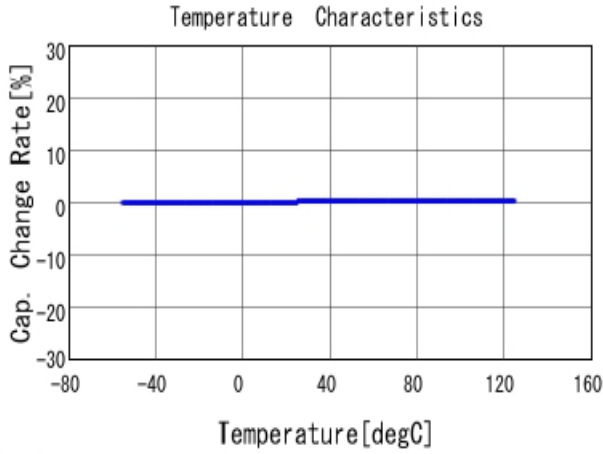
■ GJM0335C1HR90WB01 C-Temp. capchange, DCOV, AC1Vrms
