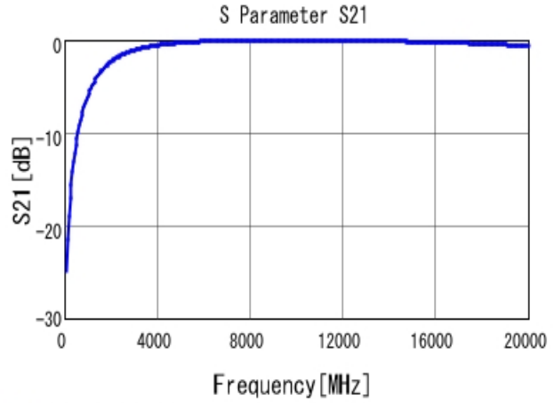
■ GJM0335C1HR90WB01 S21 DCOV, 25degC
