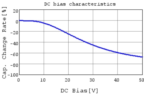
GRT32DC81H335KE01 C-DC bias capchange, 25.0c
