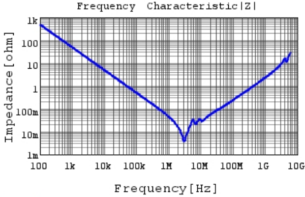
GRT32DC81H335KE01 |Z| DCOV, 25degC
