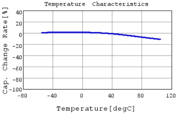
GRT32DC81H335KE01 C-Temp. capchange, DC0.0V,
