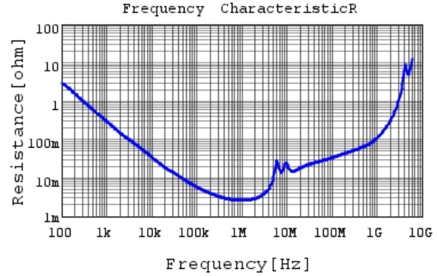
GRT32DC81H335KE01 R DCOV, 25degC
