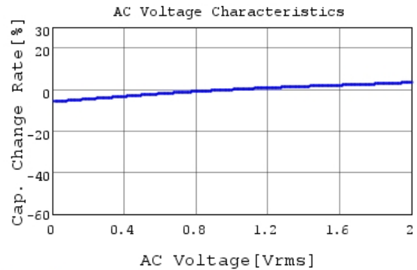
GRT32DC81H335KE01 C-AC Voltage capchange, Dc
