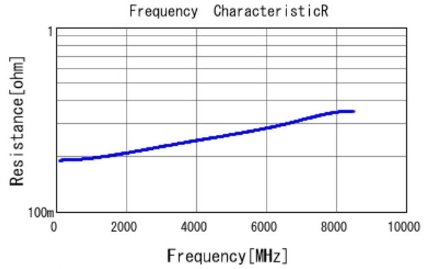
GJM1555C1H2R1BB01 R DCOV, 25degC
