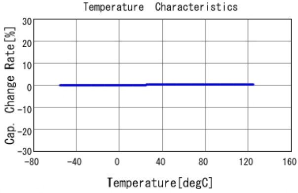
GJM1555C1H2R1BB01 C-Temp. capchange, DC0V, AC1Vrms
