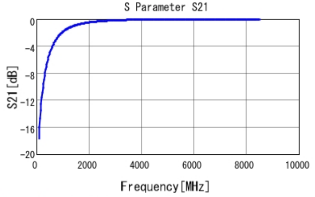
GJM1555C1H2R1BB01 S21 DC0V, 25degC
