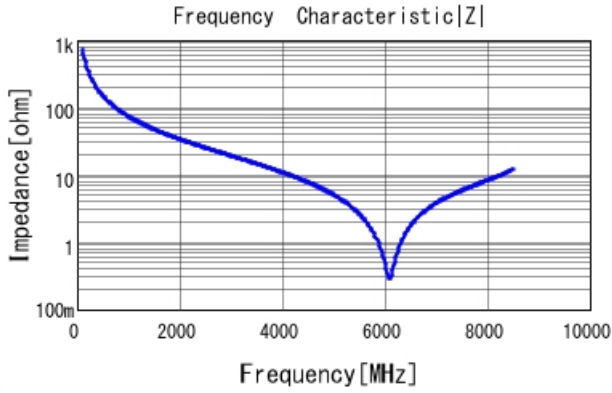
GJM1555C1H2R1BB01 |Z| DCOV, 25degC
