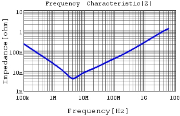
NFM15PC915R0E3 |Z| DCOV,25degC, Non-feedthro
