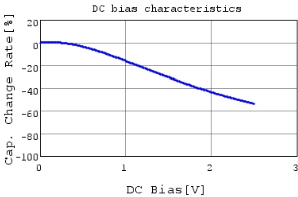
NFM15PC915R0E3 C-DC bias capchange, 25.0degC
