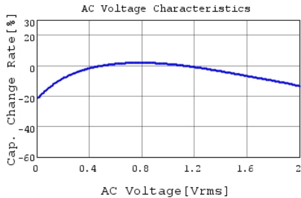
NFM15PC915R0E3 C-AC Voltage capchange, DCOV,
