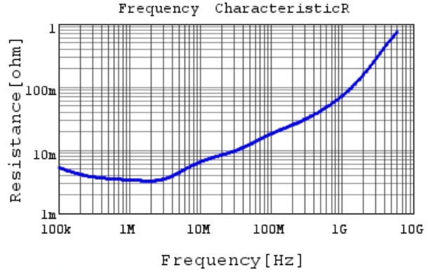
NFM15PC915R0E3 R DCOV,25degC, Non-feedthro
