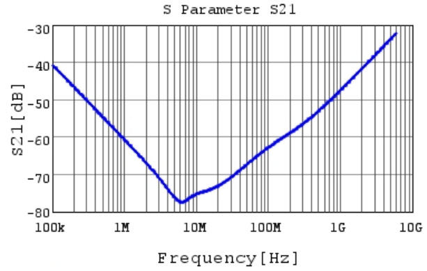
■ NFM15PC915R0E3 S21 DCOV, 25degC, Feedthrough
