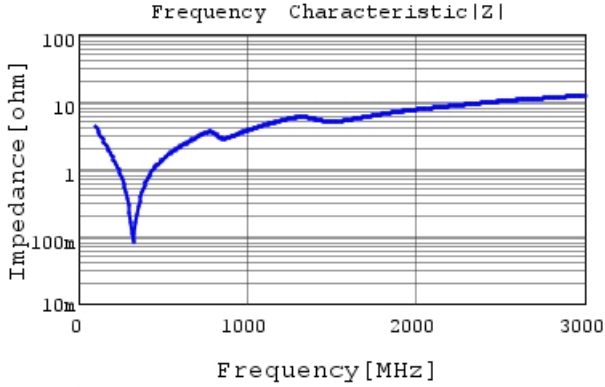
GRM31A7U2J331JW31 |Z| DC0V, 25degC
