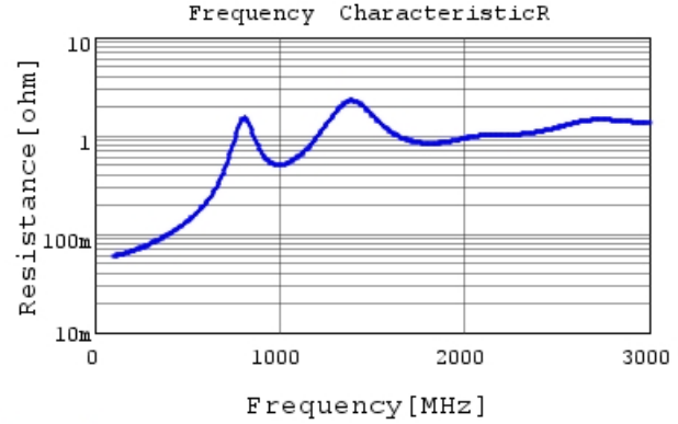
GRM31A7U2J331JW31 R DC0V, 25degC
