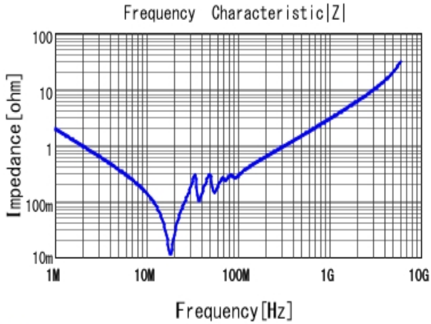
■ GRM31C2C1H823JA01 |Z| DCOV, 20degC
