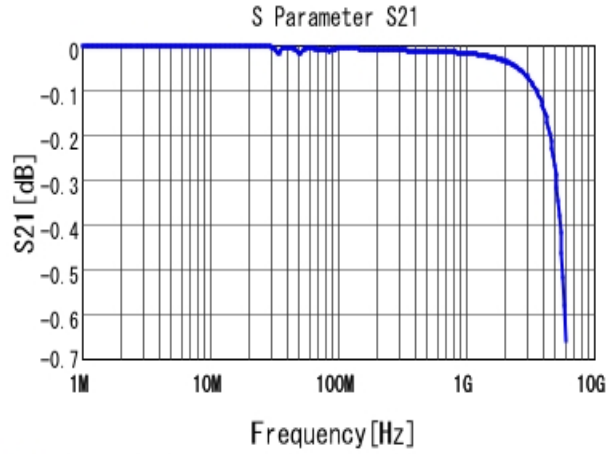
■ GRM31C2C1H823JA01 S21 DCOV, 20degC
