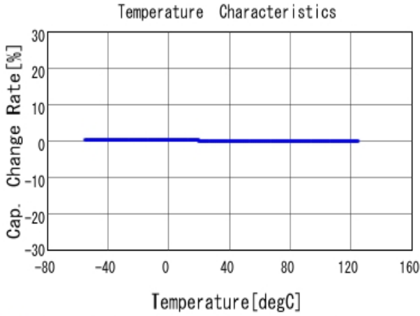
■ GRM31C2C1H823JA01 C-Temp. capchange, DCOV, AC1Vrms
