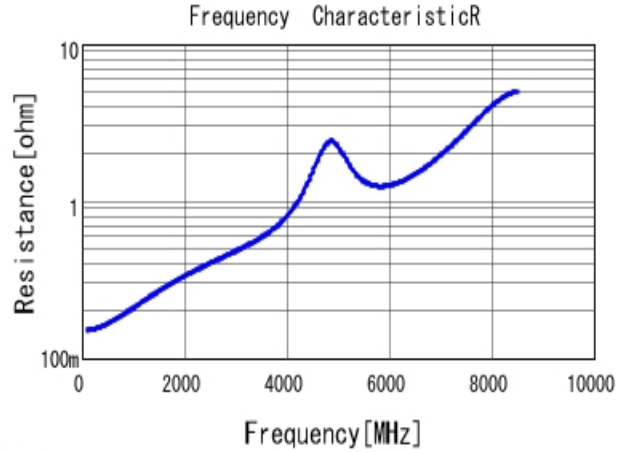
■ GRM1555C1H150JA01 R DCOV, 25degC
