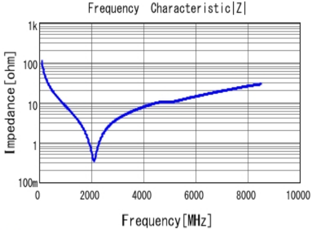
■ GRM1555C1H150JA01 |Z| DCOV, 25degC
