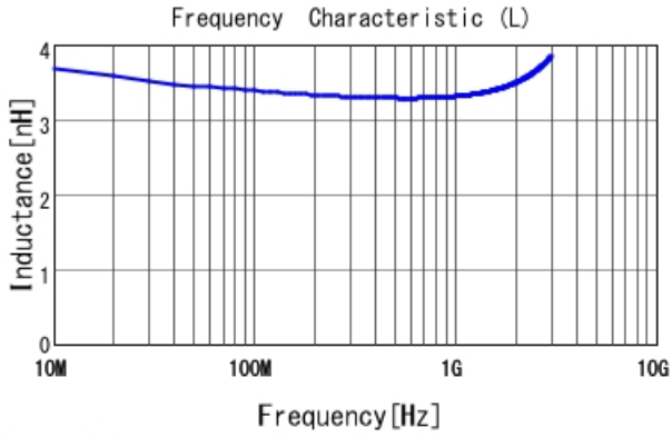
LQG15WH3N4C02 L
