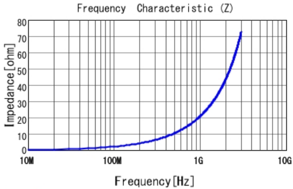
LQG15WH3N4C02 |Z|
