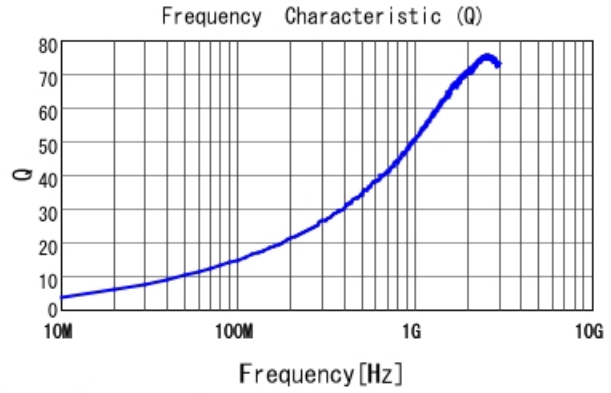
LQG15WH3N4C02 Q
