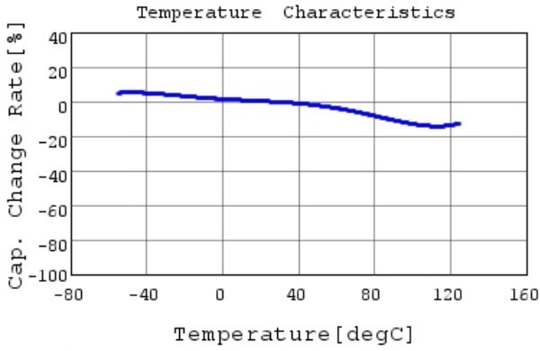
RDER72E104K2M1H03A C-Temp. capchange, DCOV,
