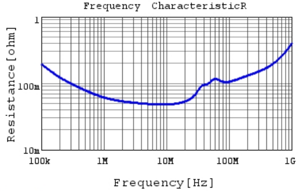
RDER72E104K2M1H03A R DCOV, 25degC
