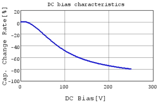
RDER72E104K2M1H03A C-DC bias capchange, 25.0
