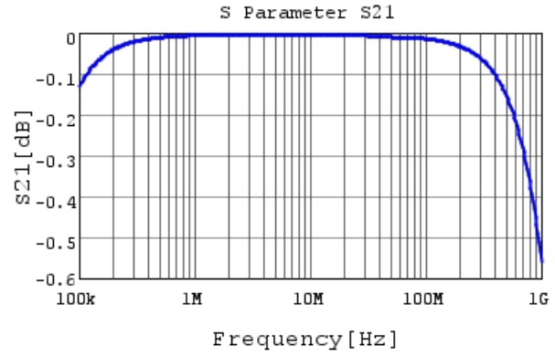
RDER72E104K2M1H03A S21 DCOV, 25degC
