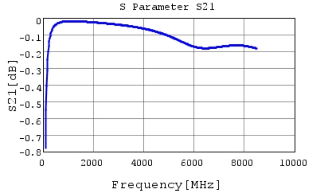
GRM0335C2A360JA01 S21 DCOV, 25degC
