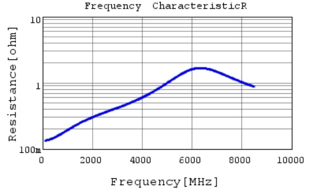
GRM0335C2A360JA01 R DCOV, 25degC
