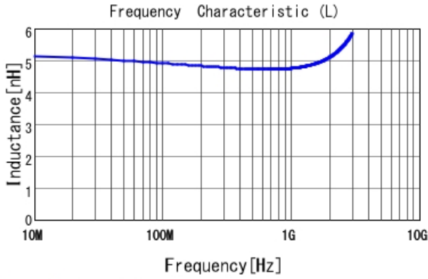
LQP03TG4N7J02 L
