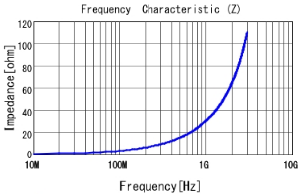
LQP03TG4N7J02 |Z|
