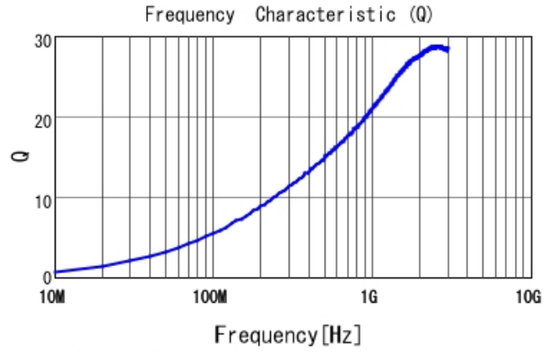
LQP03TG4N7J02 Q
