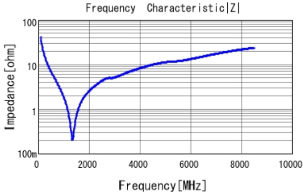
GRM1555C2A390JA01 |Z| DCOV, 25degC
