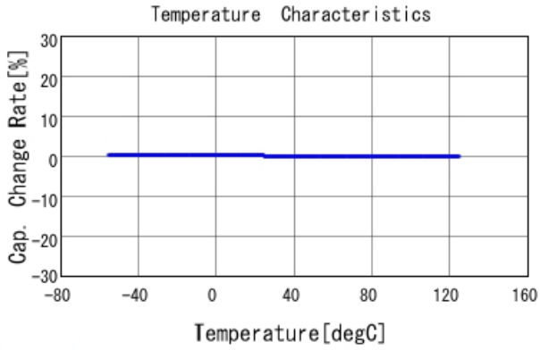
GRM1555C2A390JA01 C-Temp. capchange, DCOV, AC1Vrms
