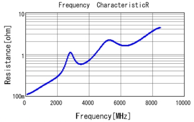
GRM1555C2A390JA01 R DCOV, 25degC
