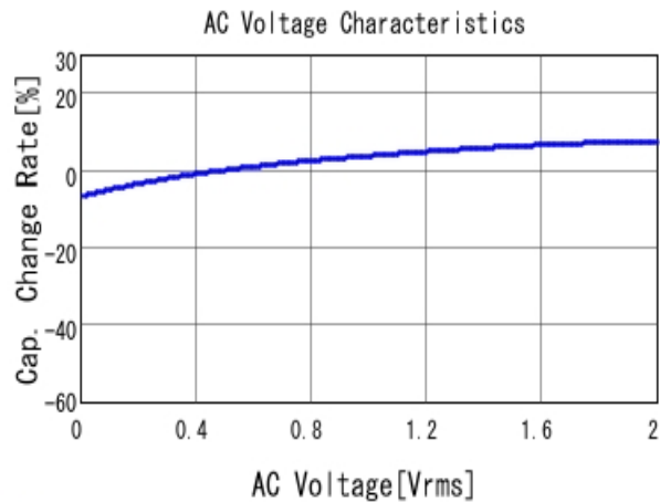
■ GRM155R61A154KE19 C-AC Voltage capchange, DCOV, 25.0d
