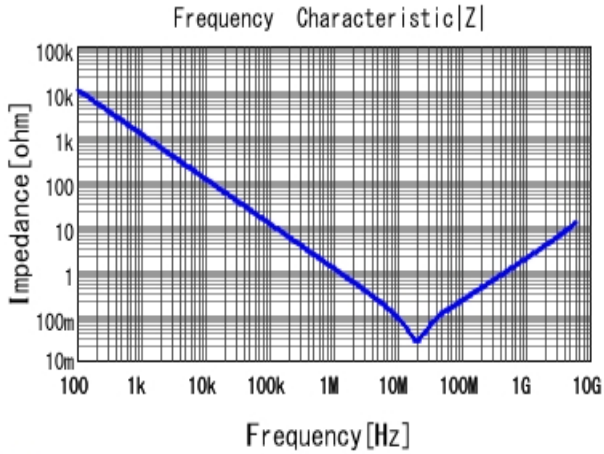
■ GRM155R61A154KE19 |Z| DCOV, 25degC
