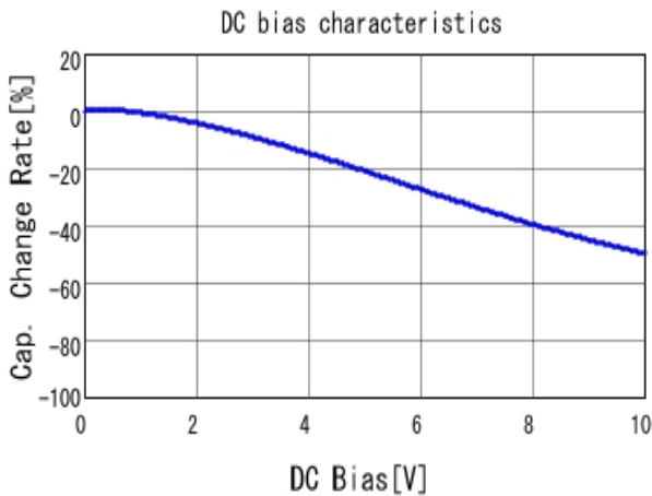
■ GRM155R61A154KE19 C-DC bias capchange, 25.0degC, AC0.
