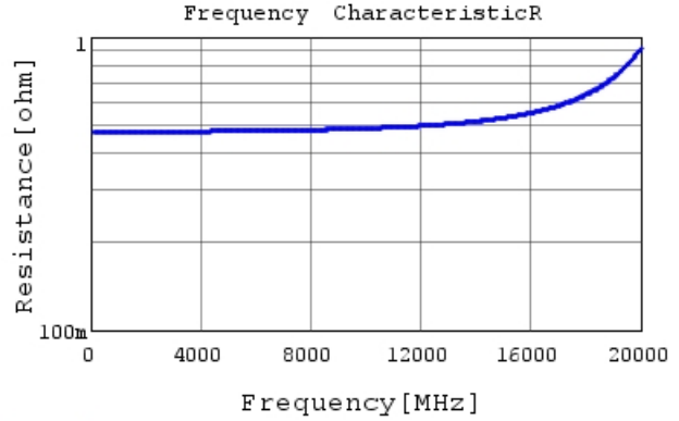
GCQ1555C1HR20WB01 R DC0V, 25degC
