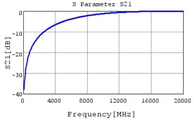
GCQ1555C1HR20WB01 S21 DCOV, 25degC
