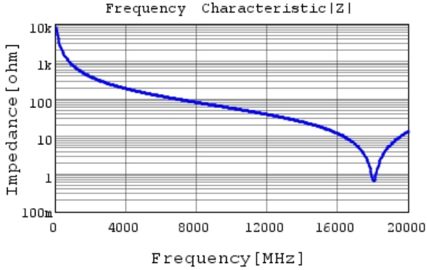
GCQ1555C1HR20WB01 |Z| DC0V, 25degC
