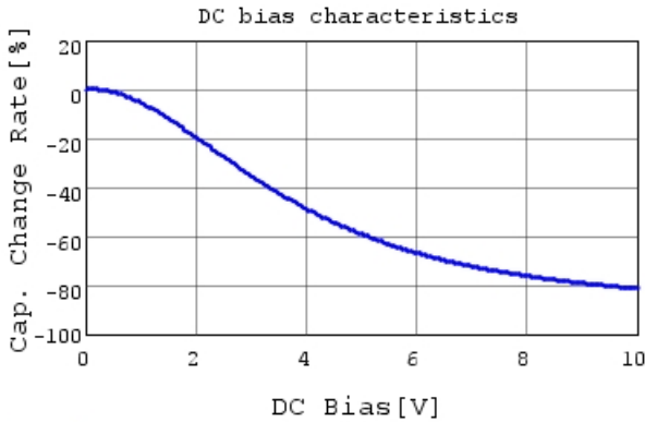
GRM155D71A225ME15 C-DC bias capchange, 25.0c
