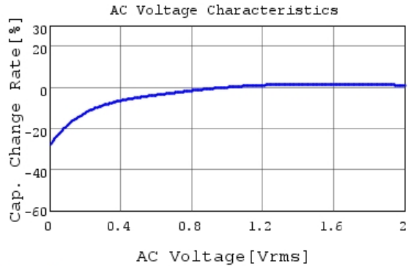
GRM155D71A225ME15 C-AC Voltage capchange, Dc
