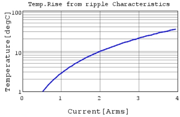
GRM155D71A225ME15 Temp.rise 1MHz
