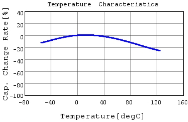
GRM155D71A225ME15 C-Temp. capchange, DC0.0V,
