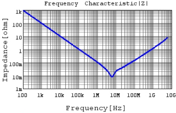
GRM155D71A225ME15 |Z| DCOV, 25degC
