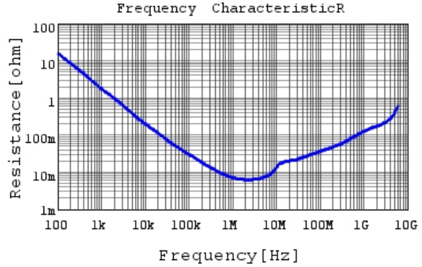
GRM155D71A225ME15 R DCOV, 25degC
