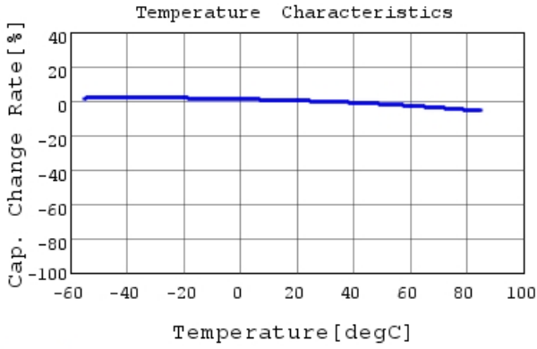
GRM033R61A332KA01 C-Temp. capchange, DC0.0V,
