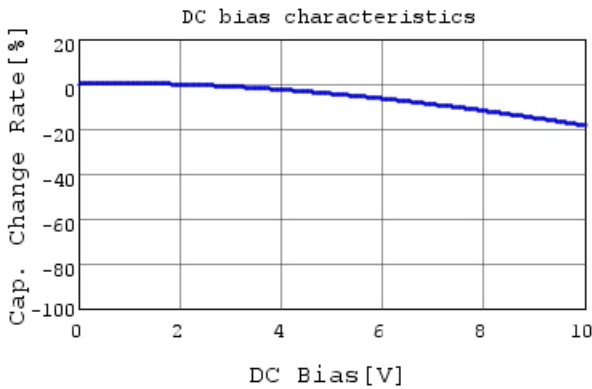
GRM033R61A332KA01 C-DC bias capchange, 25.0c
