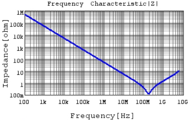
GRM033R61A332KA01 |Z| DCOV, 25degC
