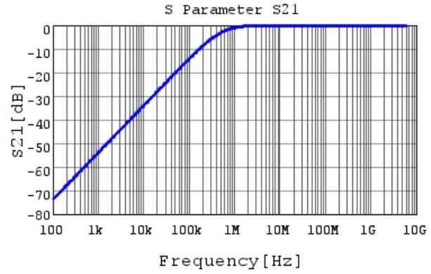
GRM033R61A332KA01 S21 DC0V,25degC
