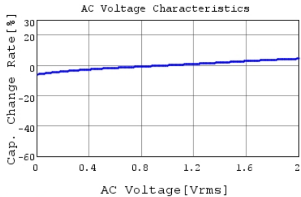
GRM033R61A332KA01 C-AC Voltage capchange, Dc
