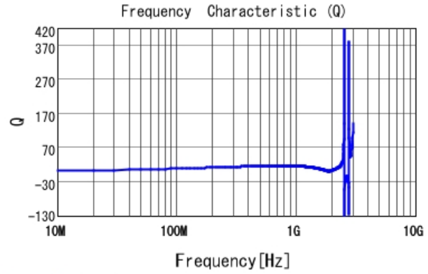
LQP03TN51NHZ2 Q
