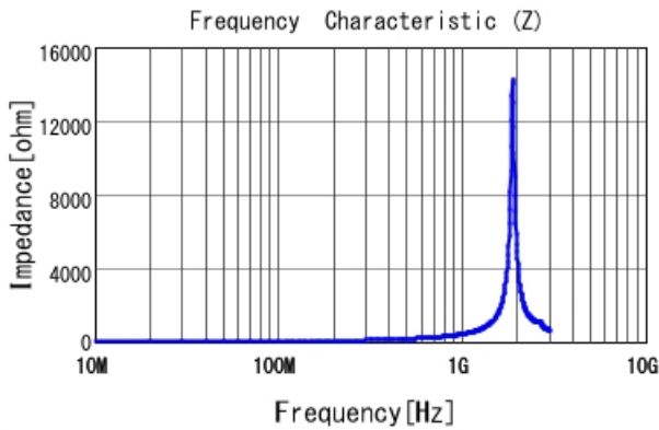
LQP03TN51NHZ2 |Z|
