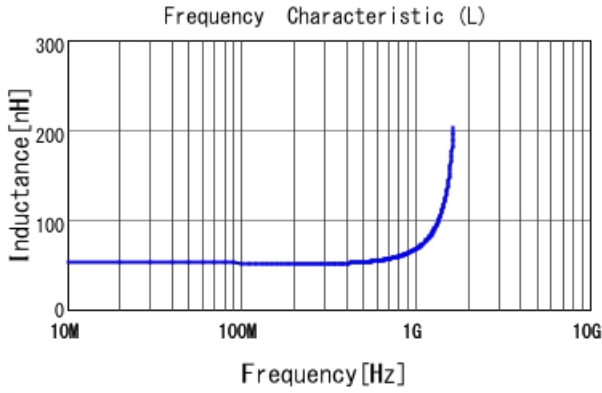
LQP03TN51NHZ2 L
