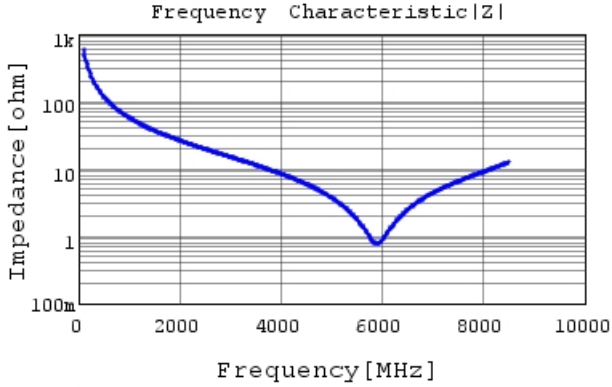
GRM0335C1H2R7CA01 |Z| DC0V, 25degC
