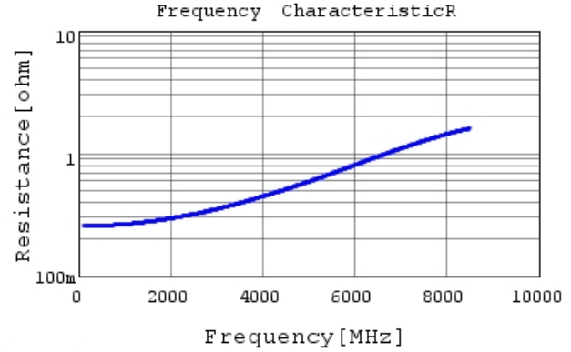
GRM0335C1H2R7CA01 R DC0V, 25degC
