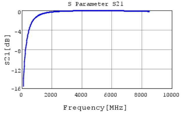
GRM0335C1H2R7CA01 S21 DCOV, 25degC
