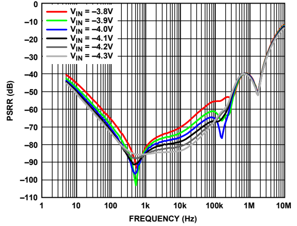
Figure 33. Power Supply Rejection Ratio (PSRR) vs. Frequency at Various Input Voltages, V_{OUT} = -3.3V , I_{LOAD} = -500mA
