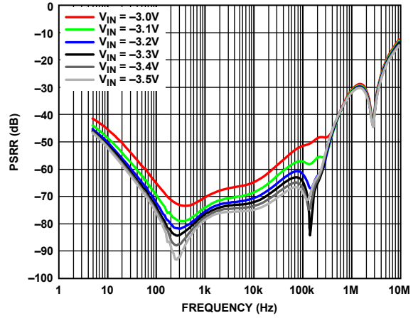
Figure 32. Power Supply Rejection Ratio (PSRR) vs. Frequency at Various Input Voltages, V_{OUT} = -2.5V , I_{LOAD} = -500mA
