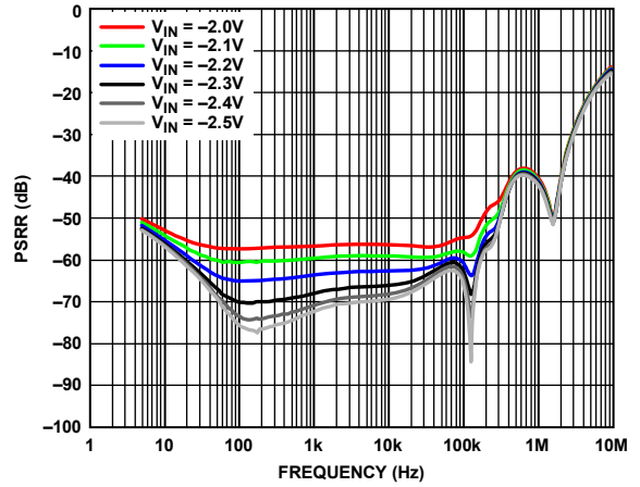
Figure 31. Power Supply Rejection Ratio (PSRR) vs. Frequency at Various Input Voltages, V_{OUT} = -1.2V , I_{LOAD} = -500mA
