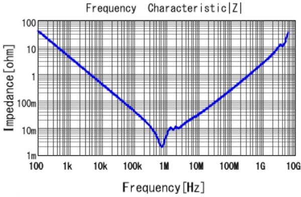
■ GRM32EC81A476ME19 |Z| DCOV, 25degC
