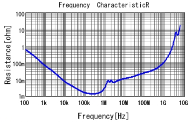
■ GRM32EC81A476ME19 R DCOV, 25degC
