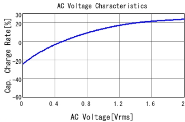
■ GRM32EC81A476ME19 C-AC Voltage capchange, DCOV, 25.0d
