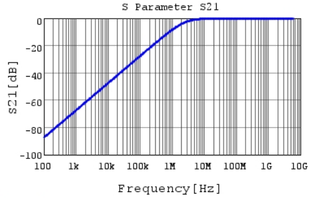
GRM033R61E681KA01 S21 DCOV,25degC
