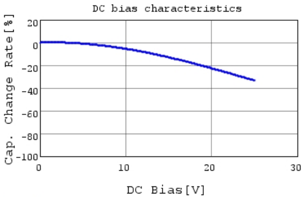
GRM033R61E681KA01 C-DC bias capchange, 25.0c
