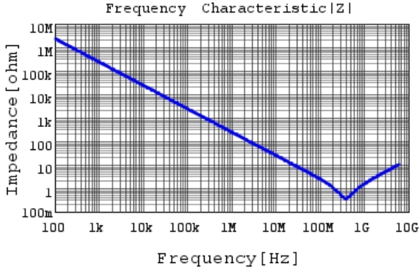
GRM033R61E681KA01 |Z| DCOV, 25degC
