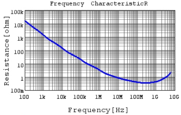
GRM033R61E681KA01 R DCOV, 25degC
