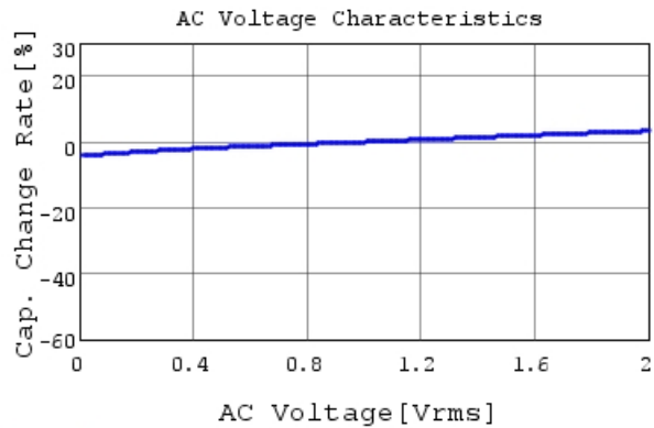
GRM033R61E681KA01 C-AC Voltage capchange, Dc
