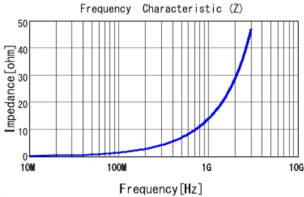
LQG15HN2N2S02 |Z|
