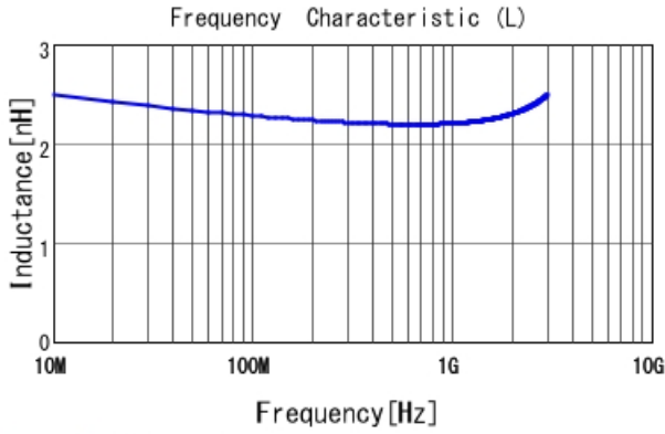
LQG15HN2N2S02 L
