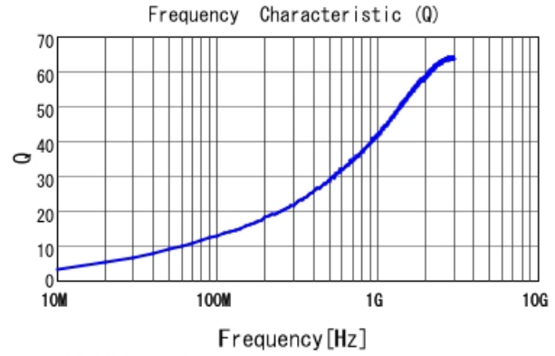
LQG15HN2N2S02 Q
