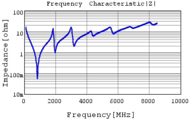
GQM1875C2E101GB12 |Z| DC0V, 25degC
