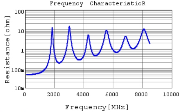
GQM1875C2E101GB12 R DC0V, 25degC
