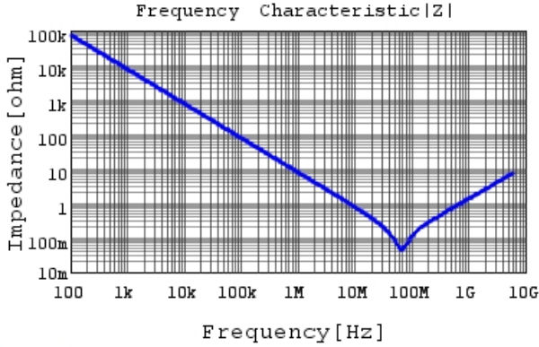
GRM033R61C223KE84 |Z| DCOV, 25degC
