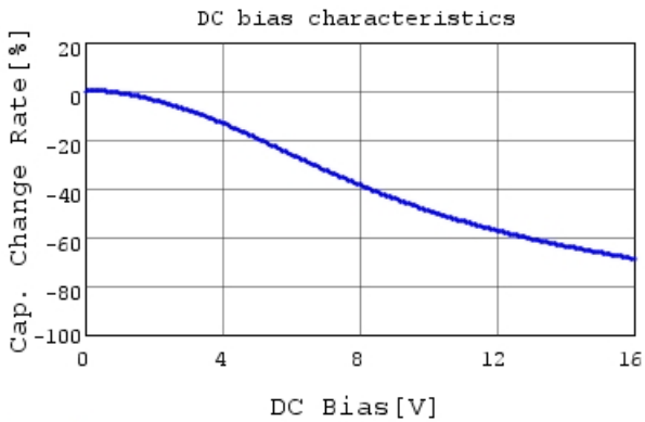
GRM033R61C223KE84 C-DC bias capchange, 25.0c
