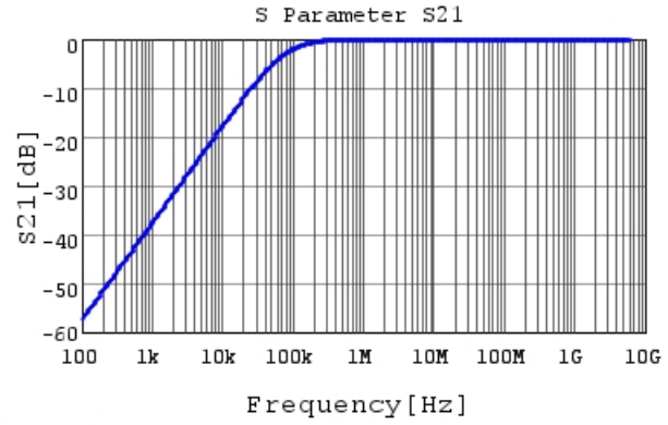
GRM033R61C223KE84 S21 DC0V, 25degC
