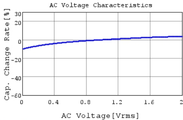
GRM033R61C223KE84 C-AC Voltage capchange, Dc
