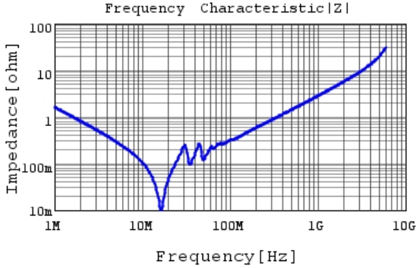
GRM31C5C1H104JA01 |Z| DC0V, 25degC
