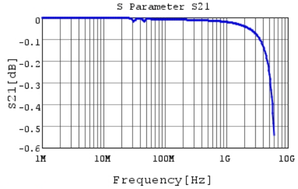
GRM31C5C1H104JA01 S21 DCOV, 25degC
