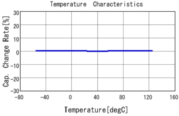
GRM1555C1H2R4CA01 C-Temp. capchange, DCOV, AC1Vrms
