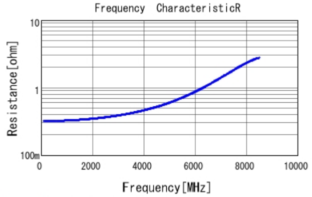
GRM1555C1H2R4CA01 R DCOV, 25degC
