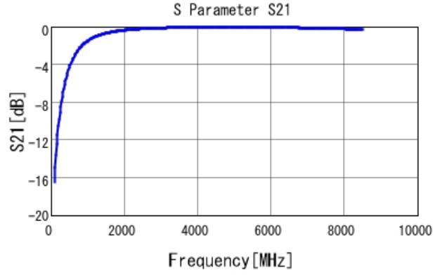
GRM1555C1H2R4CA01 S21 DCOV, 25degC
