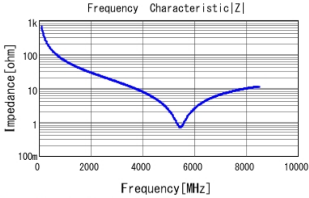
GRM1555C1H2R4CA01 |Z| DCOV, 25degC
