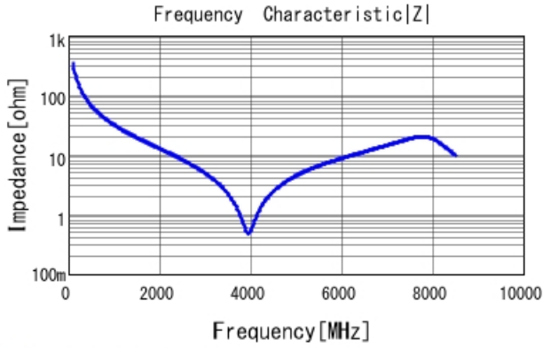
GCM1555C1H4R7WA16 |Z| DCOV, 25degC
