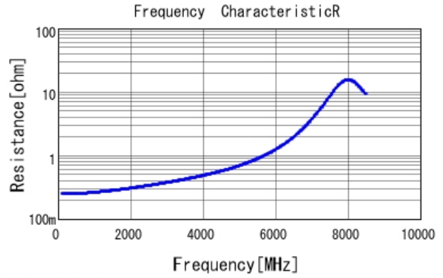
GCM1555C1H4R7WA16 R DCOV, 25degC
